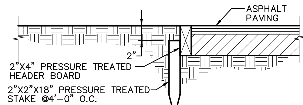
1 C1.1 HEADER BOARD NO SCALE
