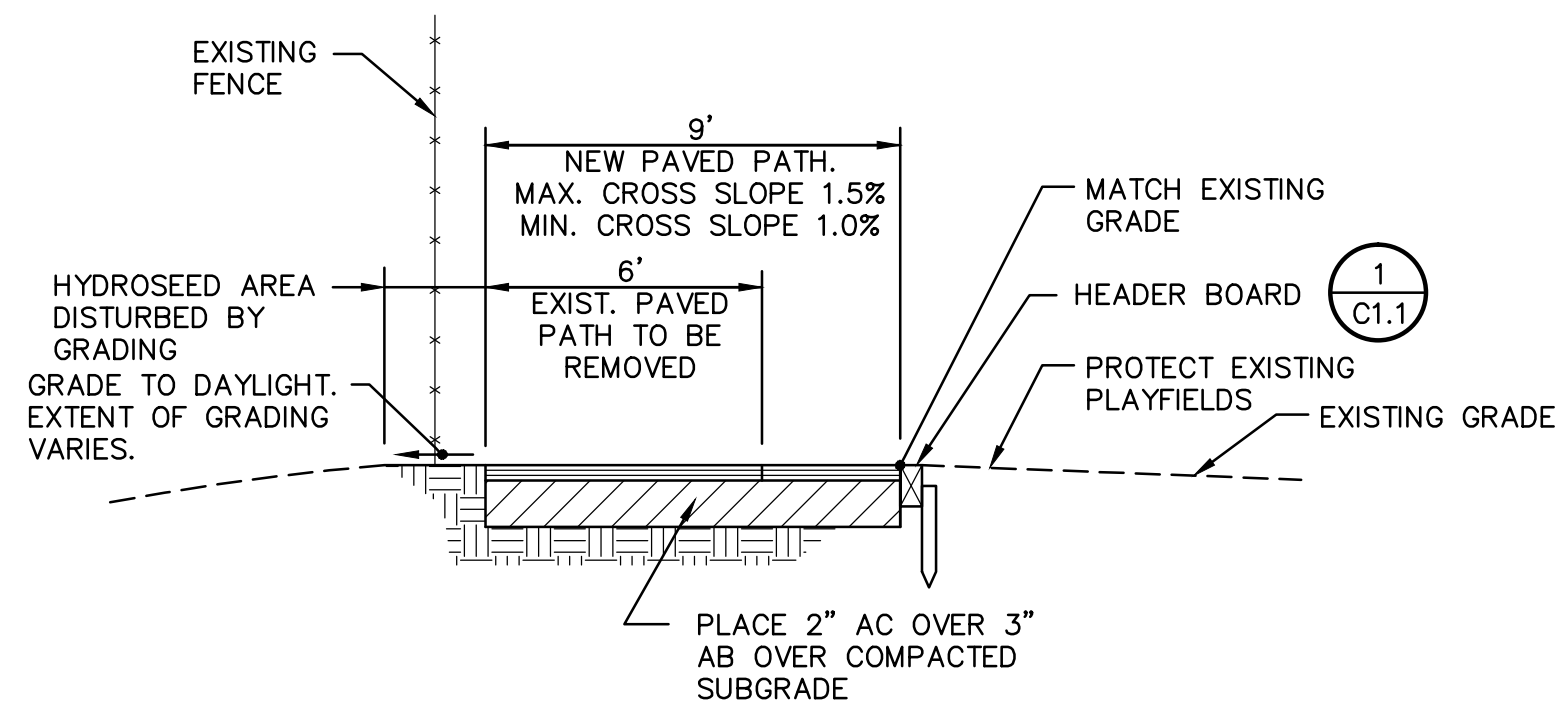
A C1.1 SECTION NO SCALE
